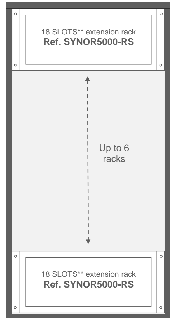
... Up to 100 EXTENSION CABINETS Ref. SYNOR5000-CS*
