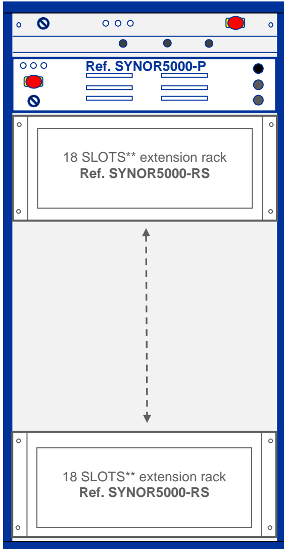
MAIN 19" CABINET Ref. SYNOR5000-C*
