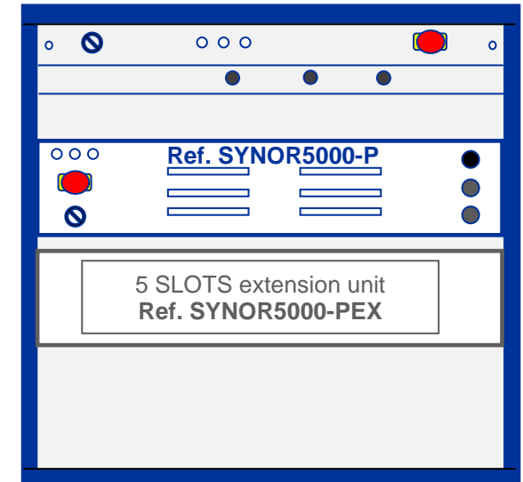
MAIN 19" CABINET Ref. SYNOR5000-C*
