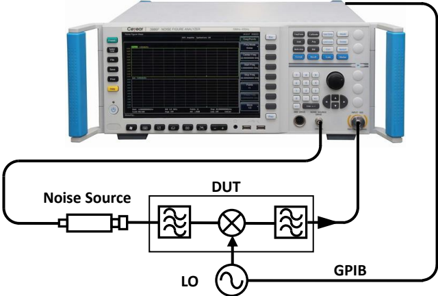
Measurement Setup
