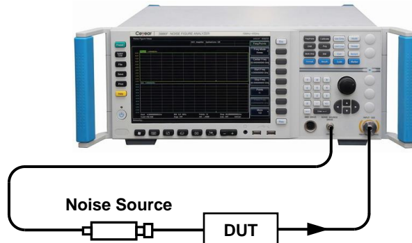
Measurement Setup
