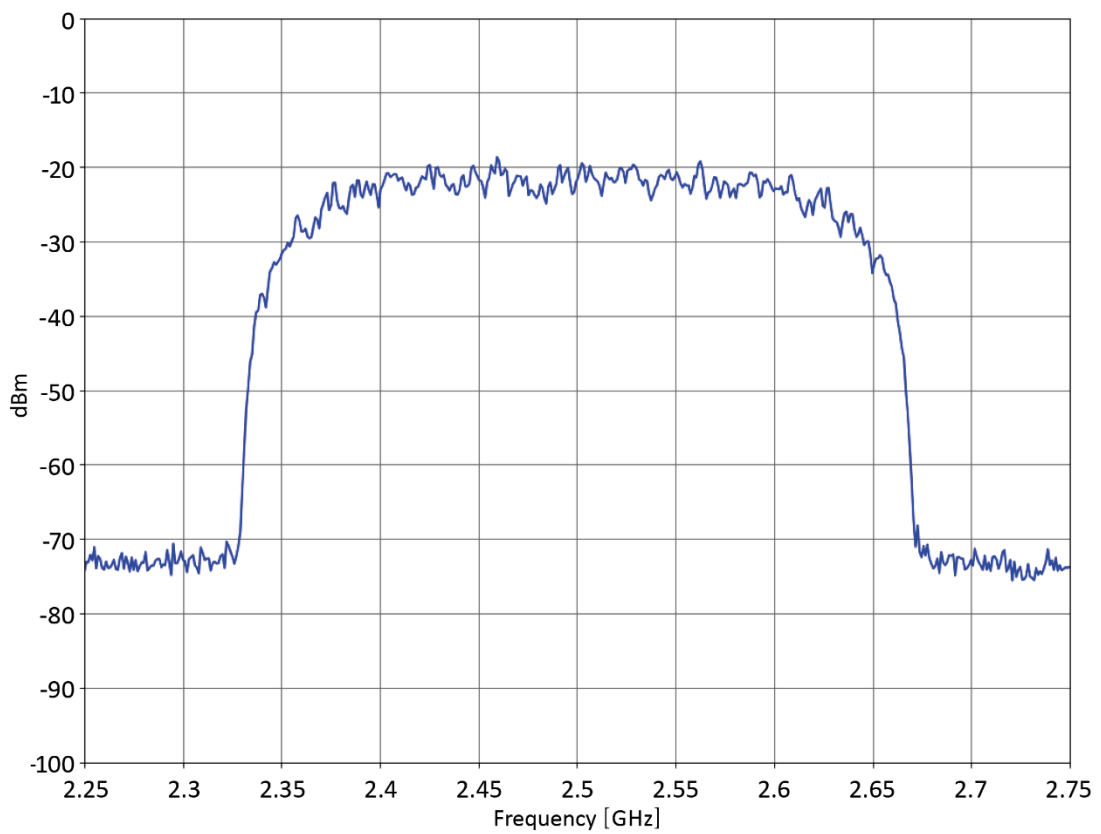
Figure 30: 16QAM 250 MS/s
