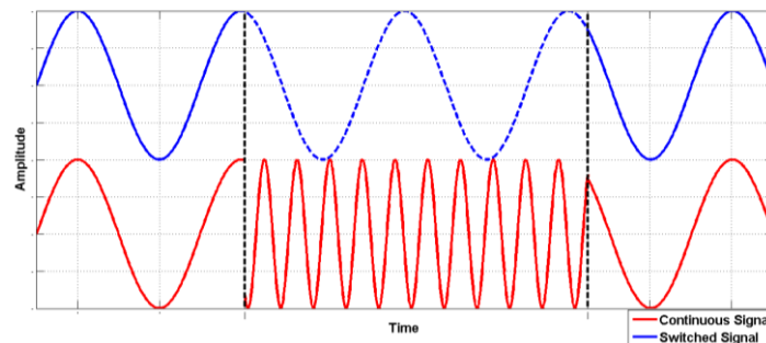
Figure 15: Phase Memory
