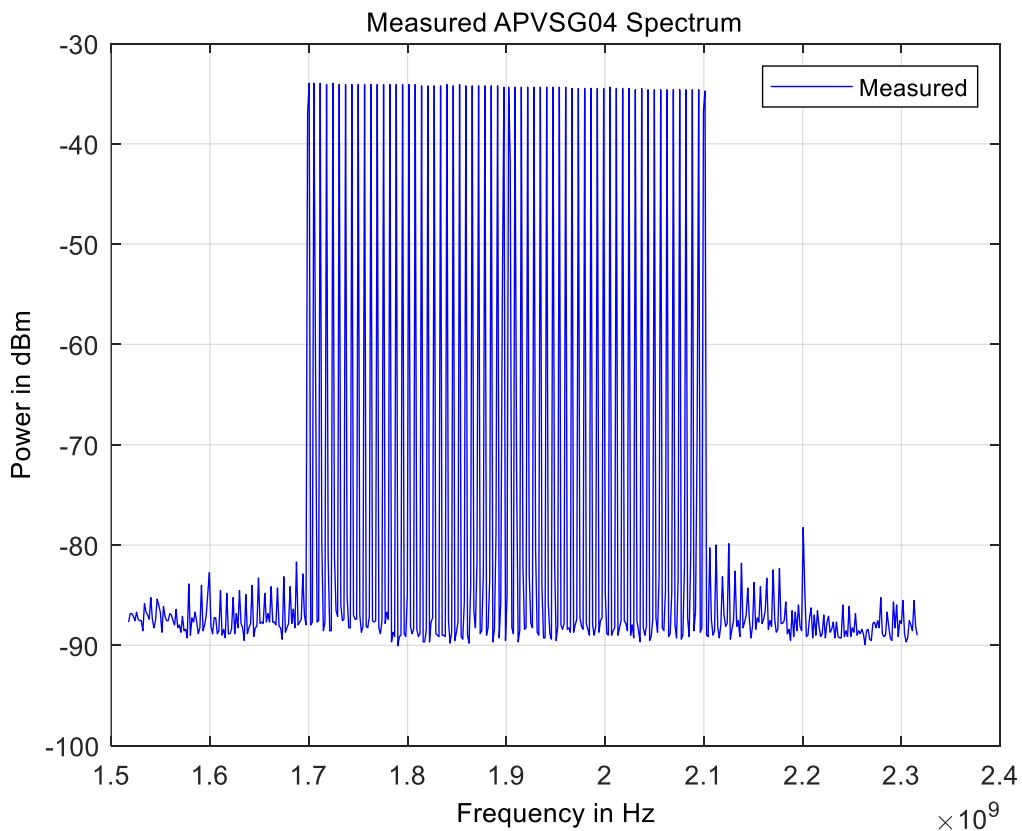
Figure 34: 64-tone 400 MHz Bandwidth Signal
