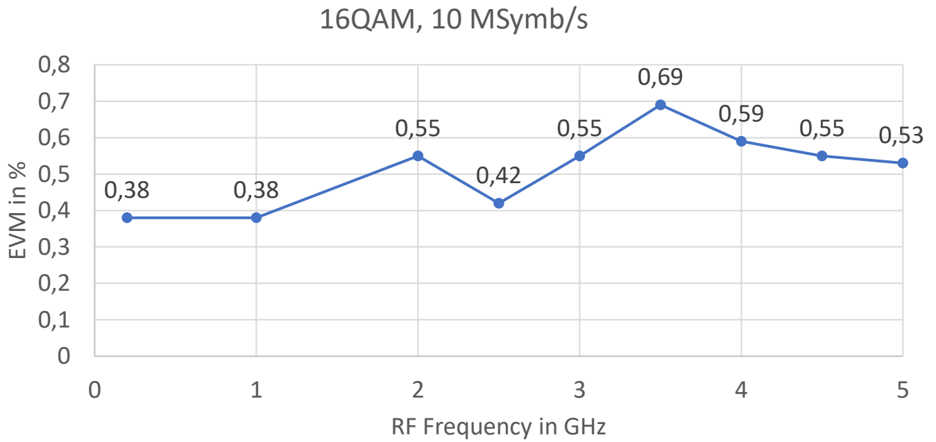
Figure 33: EMV vs RF Frequency, 16QAM, 10 Msymbols/s
