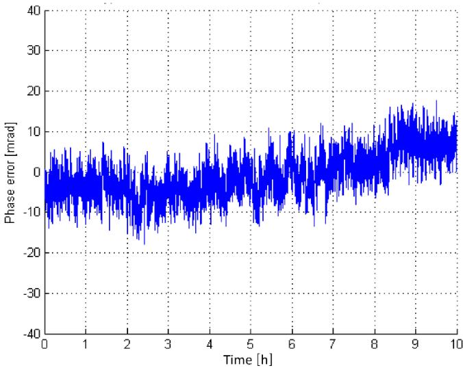
Figure 16: Phase coherence performance at 38 GHz
