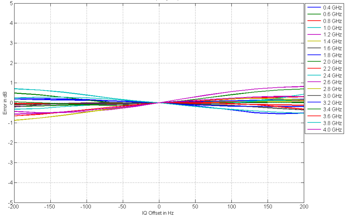
Figure 26: I/Q Relative Response (measured) APVSG04
