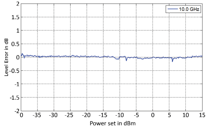
Figure 5: Power Level Accuracy APVSG12
