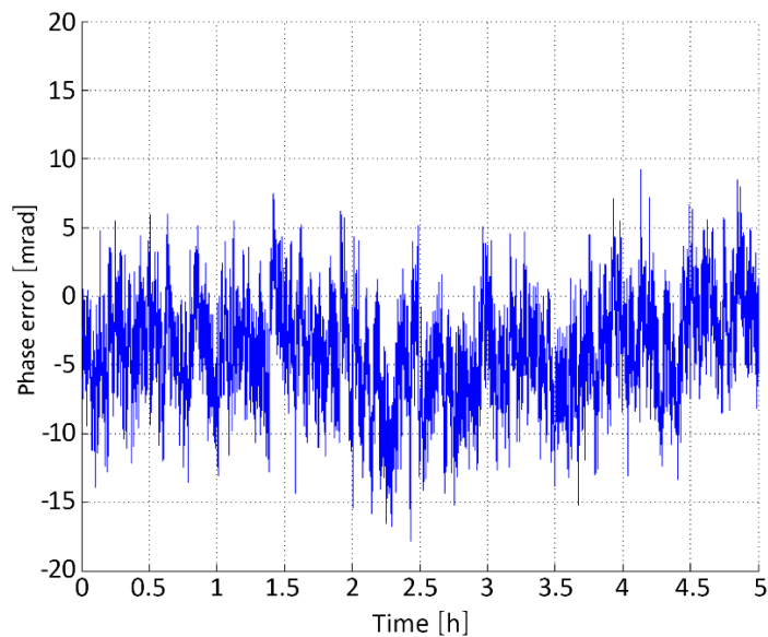
Figure 18: APVSG typical domain channel-to-channel phase error at Ch1 @0.5 GHz mixed with Ch2 @2.5 GHz VS 2 GHz from other device
