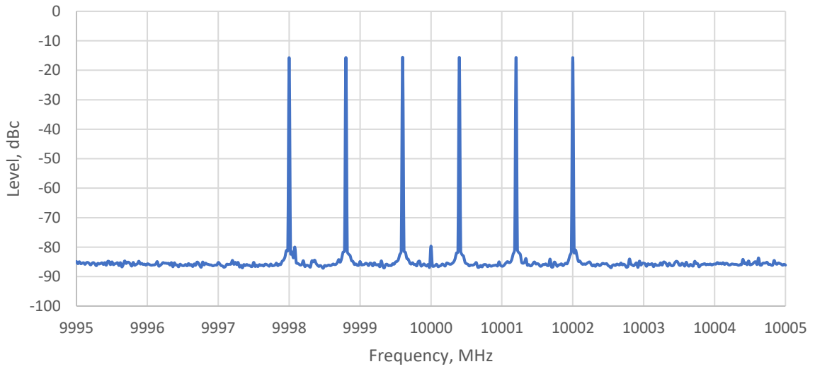
Figure 28: Carrier suppression -80 dBc for 0 dBm 6-tone signal at 10 GHz carrier
