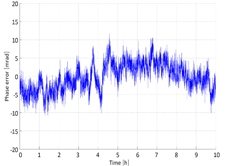
Figure 17: Phase coherence performance at 15 GHz
