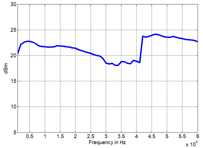
Figure 2: Maximum Output Power APVSG06
