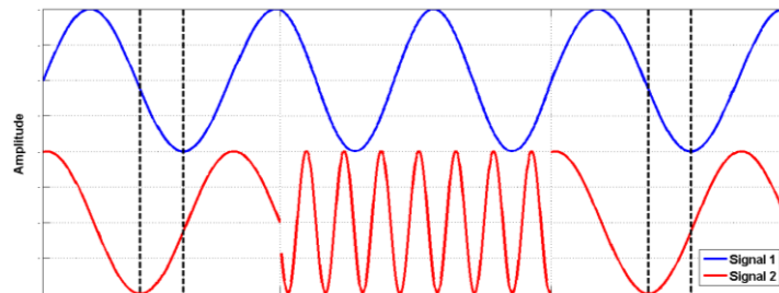
Figure 14: Phase-Coherent Switching
