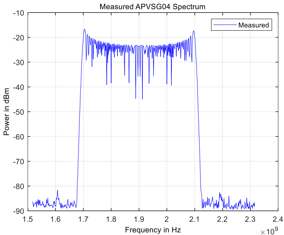
Figure 25: Wideband FM (1MHz Rate, 200 MHz Deviation)
