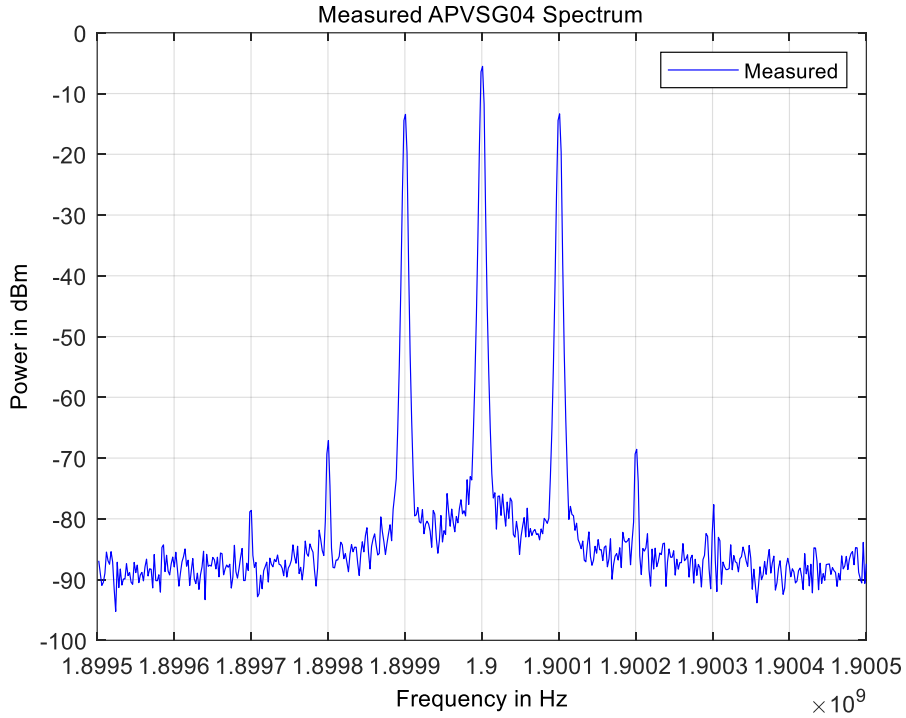
Figure 24: Amplitude Modulation (1 kHz Rate, 80% Depth)
