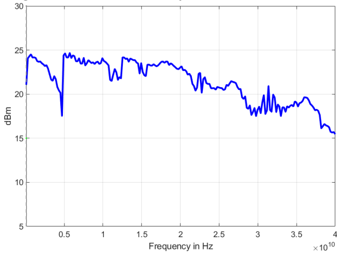
Figure 3: Maximum Output Power APVSG20/40
