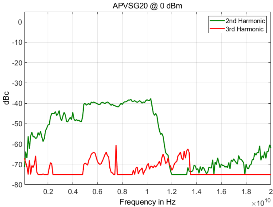
Figure 13: Harmonic Performance at Pout = 0 dBm
