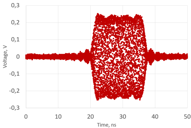
Figure 22: Pulse modulation 16 ns at 10 GHz
