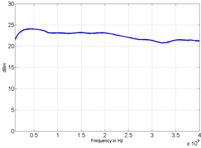
Figure 1: Maximum Output Power APVSG04
