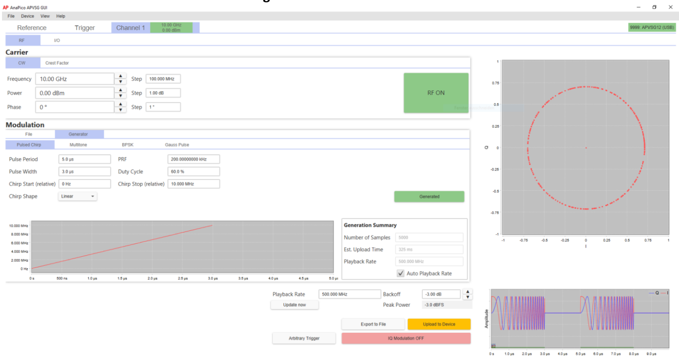
Figure 37: User Interface
