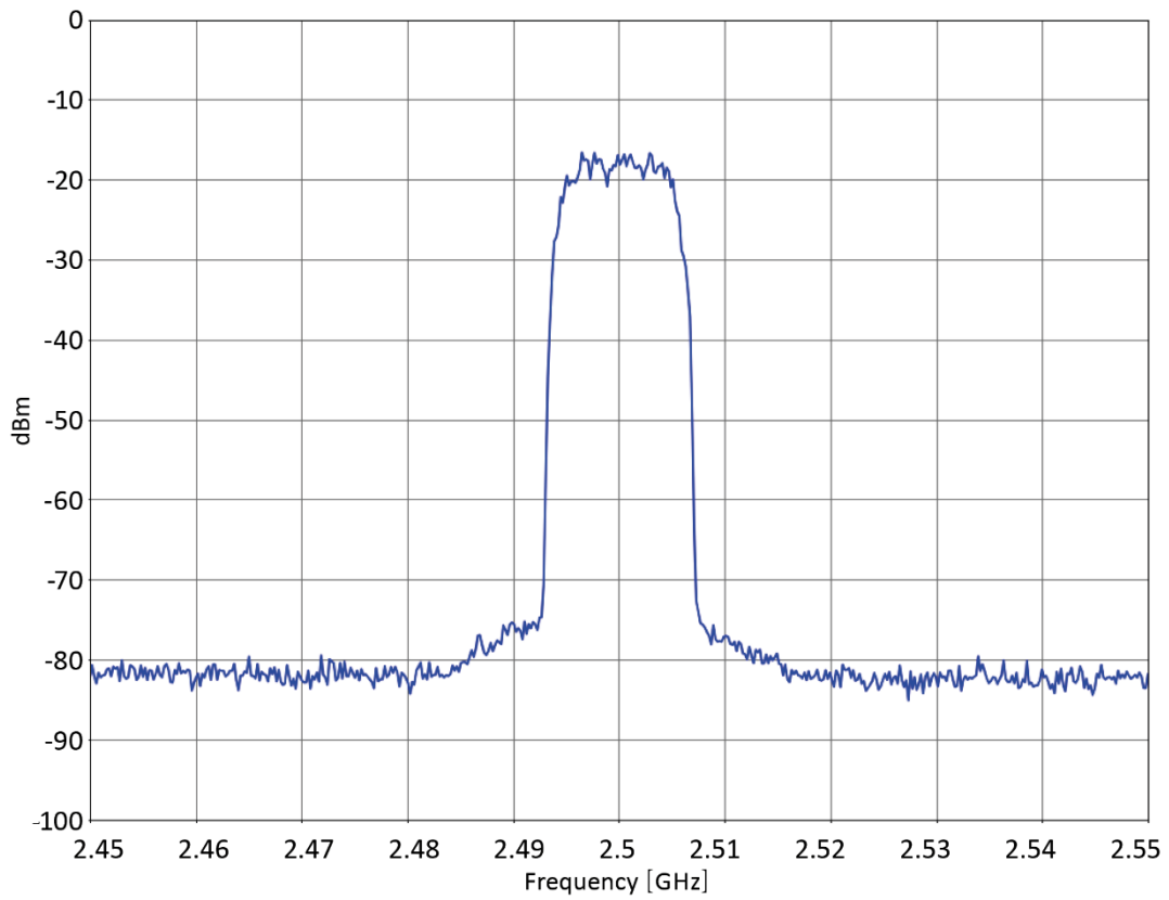
Figure 29: 256QAM 10 MS/s
