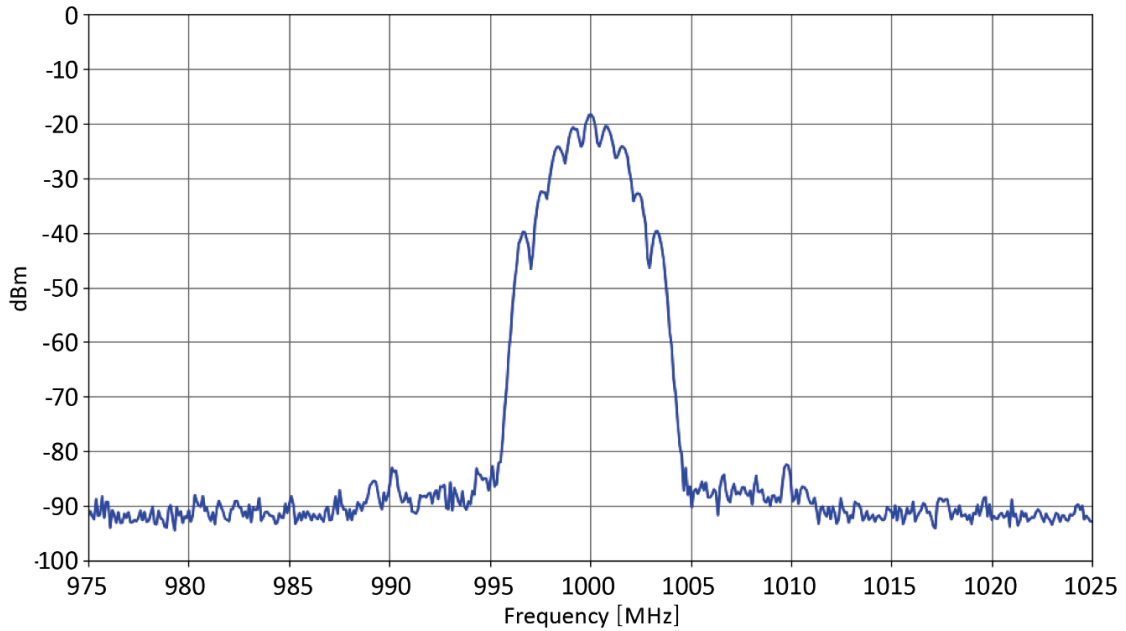
Figure 36: DME Spectrum (X Channel, Raised Cosine Filter)
