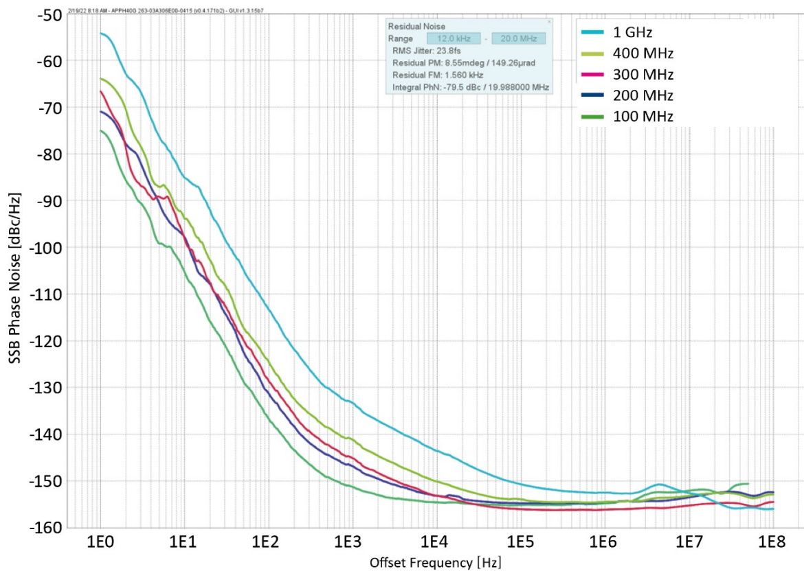
SSB Phase Noise Performance, APVSGXX, low frequency CW without option LN, Pout = 10 dBm
