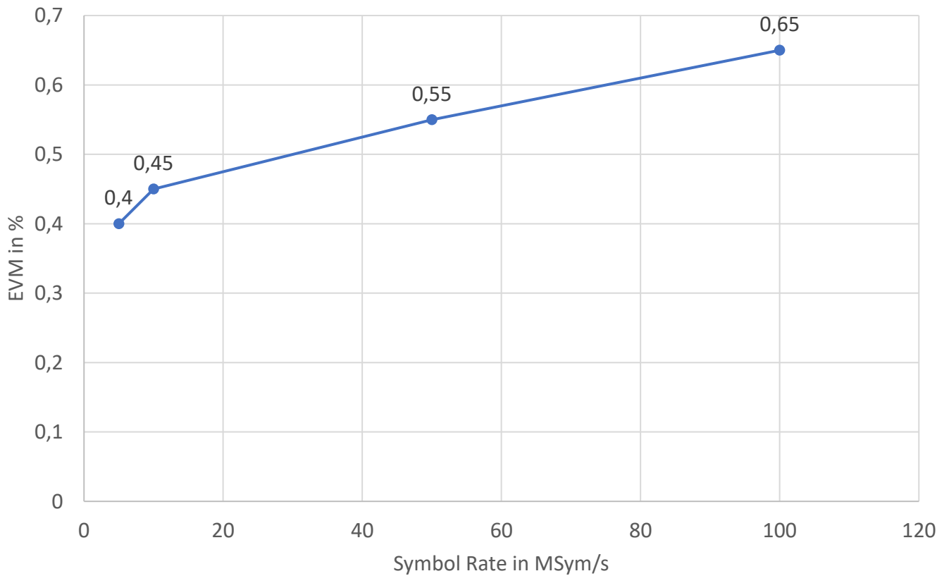
Figure 32: EMV vs Symbol Rate, 16QAM
