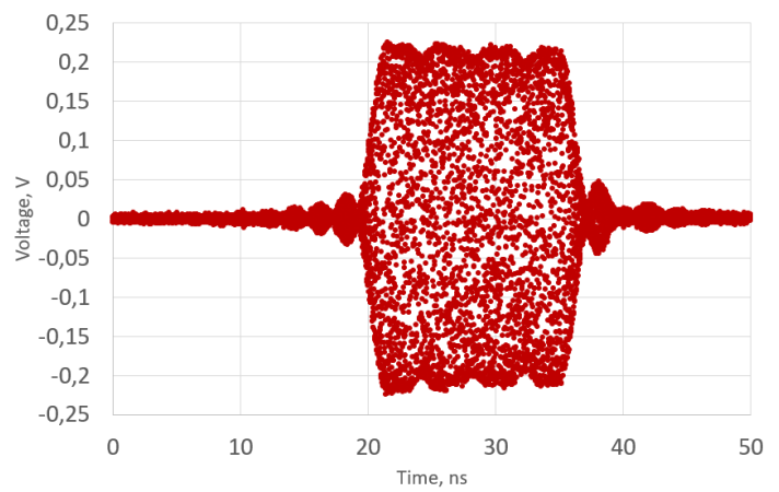
Figure 23: Pulse modulation 16 ns at 40 GHz
