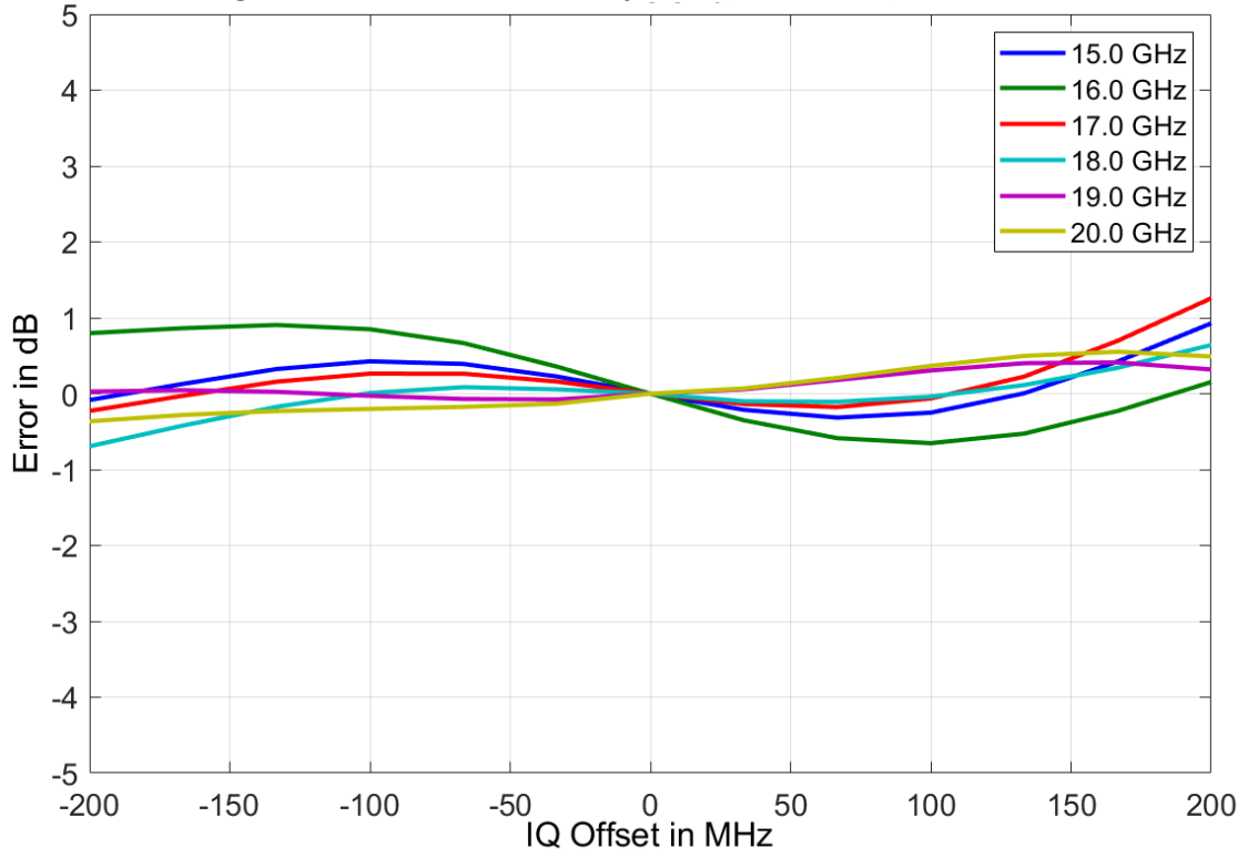
Figure 27: I/Q Relative Response (measured) APVSG20
