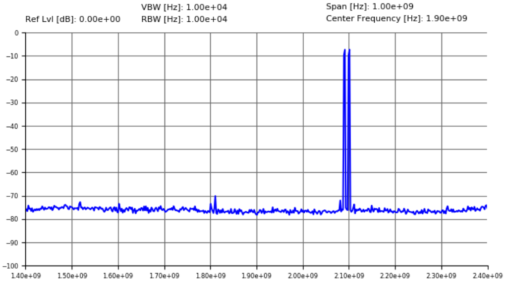
Figure 35: Two-tone Sideband Rejection
