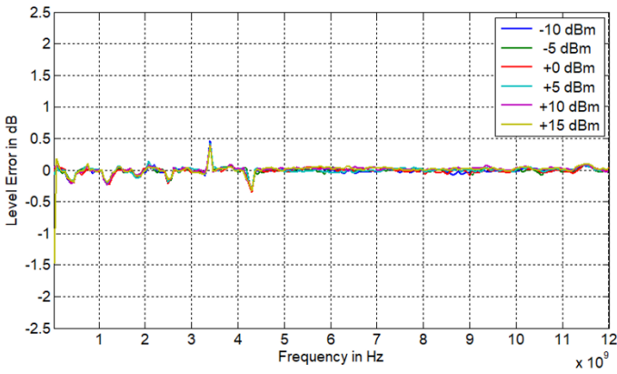
Figure 4: Power Level Accuracy APVSG12
