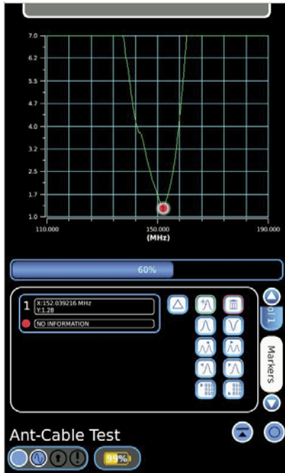
Ant-Cable Test screen showing SWR sweep
